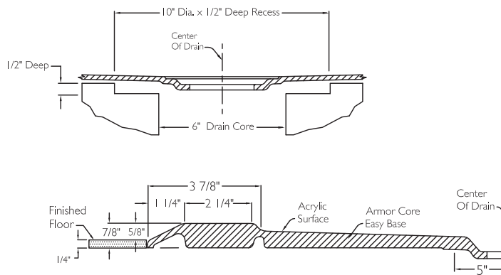
Cutaway Drain Detail
