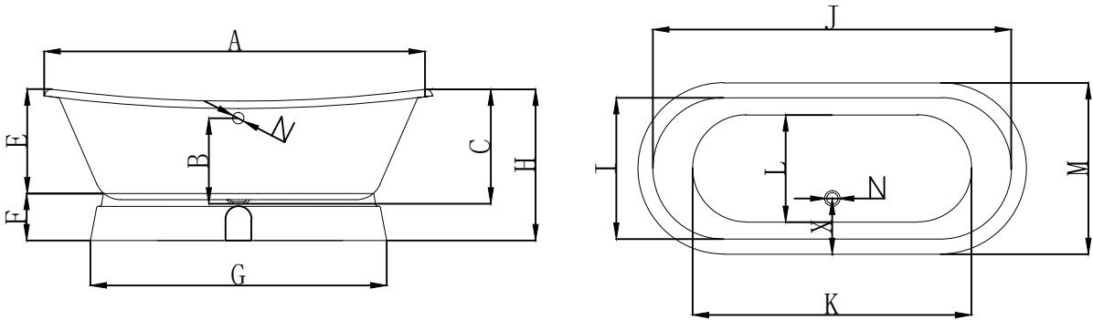
DIMENSIONS (INCHES)
