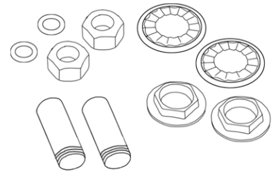
Deck Mount Hook Ups Part: T500 included in box 200 or 202
